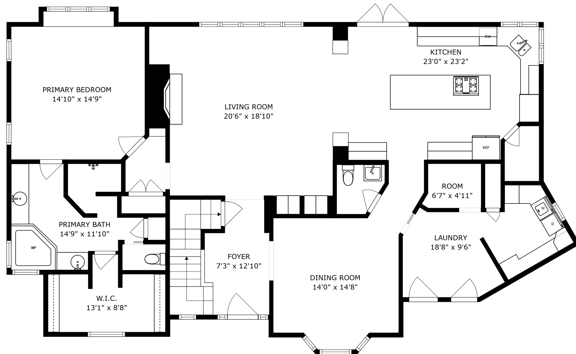
FLOOR 2
