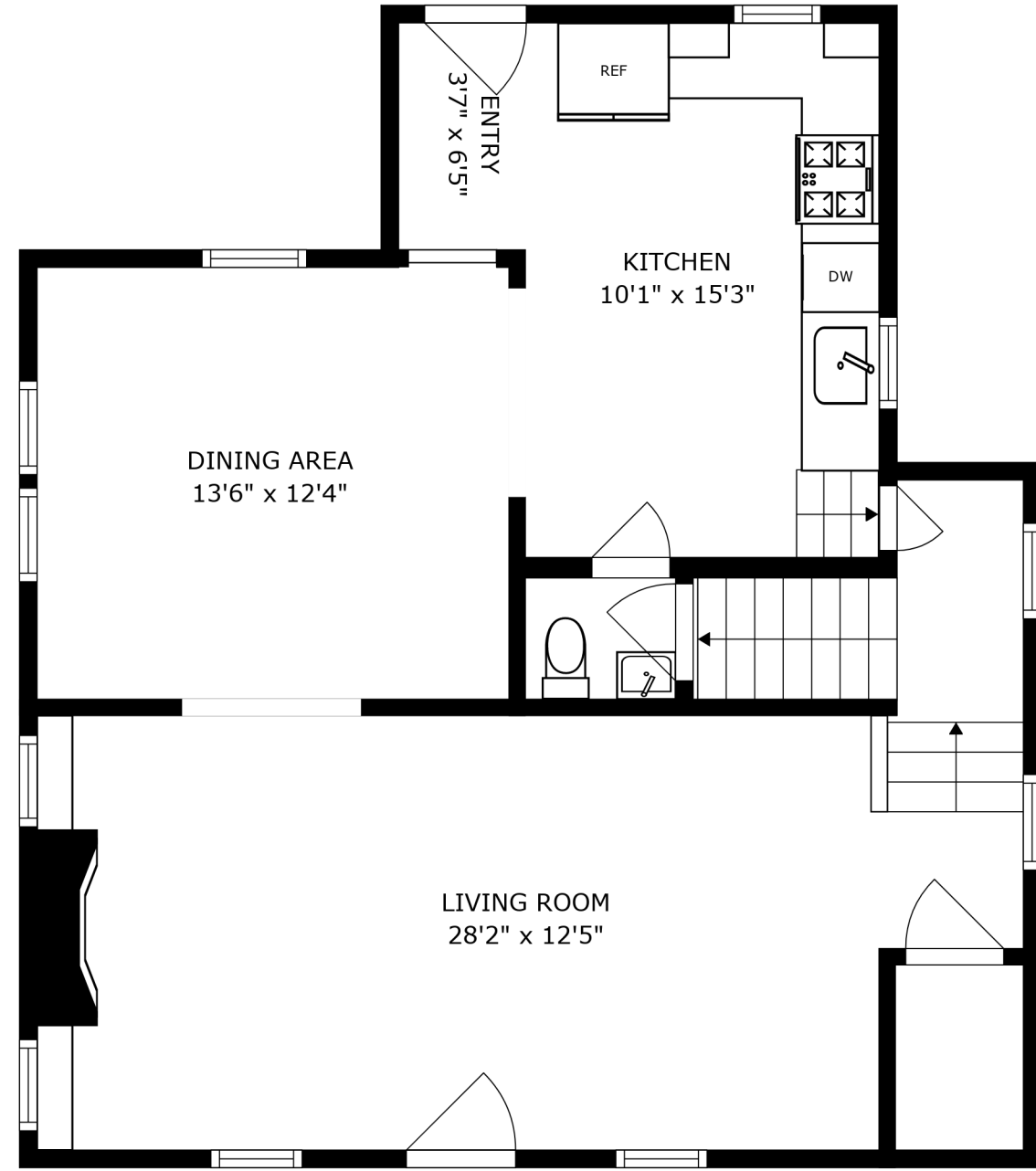
FLOOR 2
