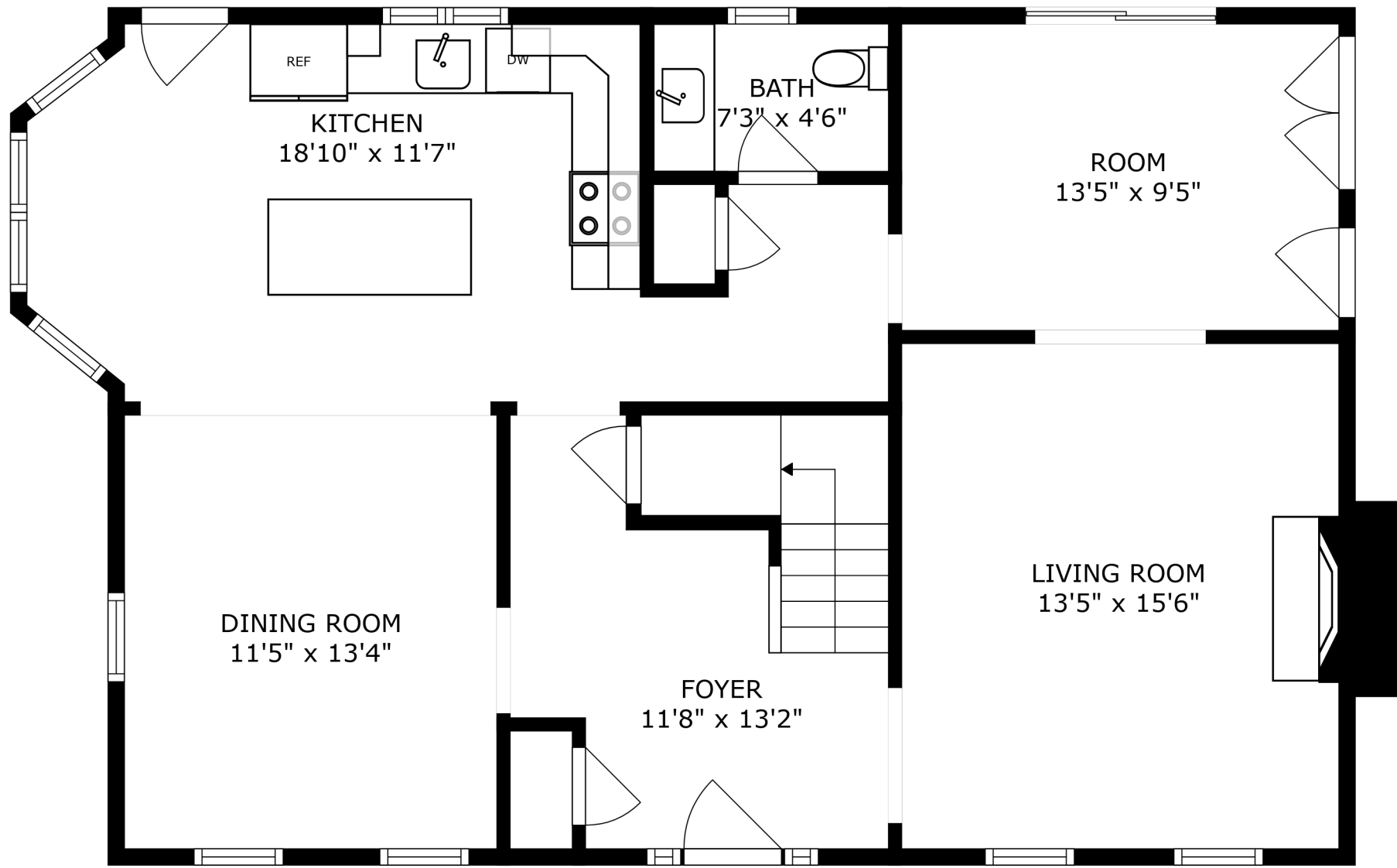
FLOOR 1
