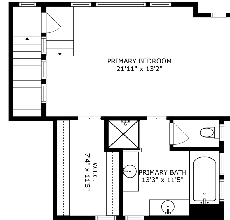
FLOOR 3
