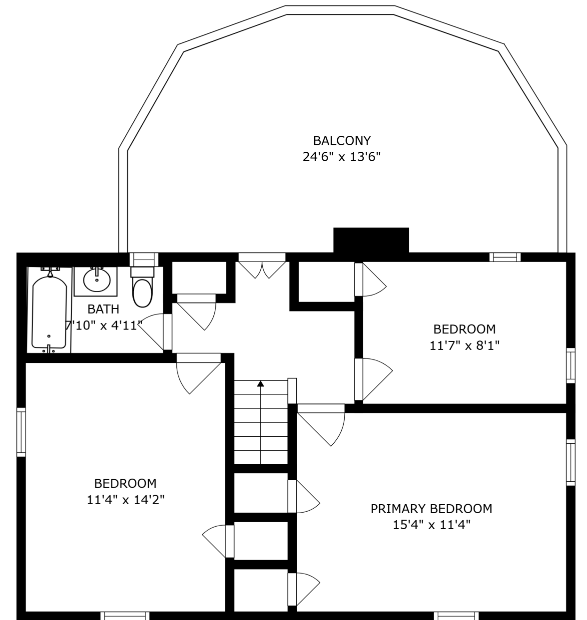
FLOOR 3
