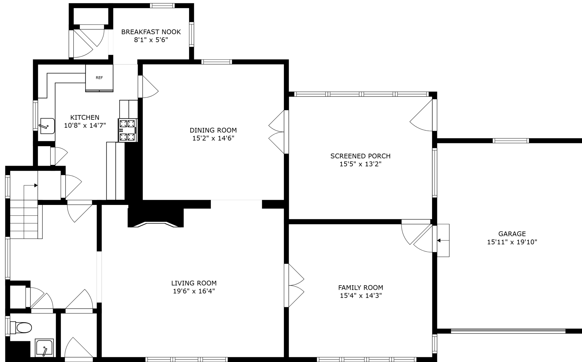
FLOOR 1
