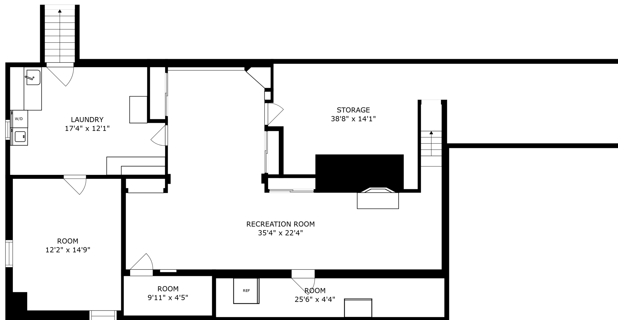
FLOOR 2
