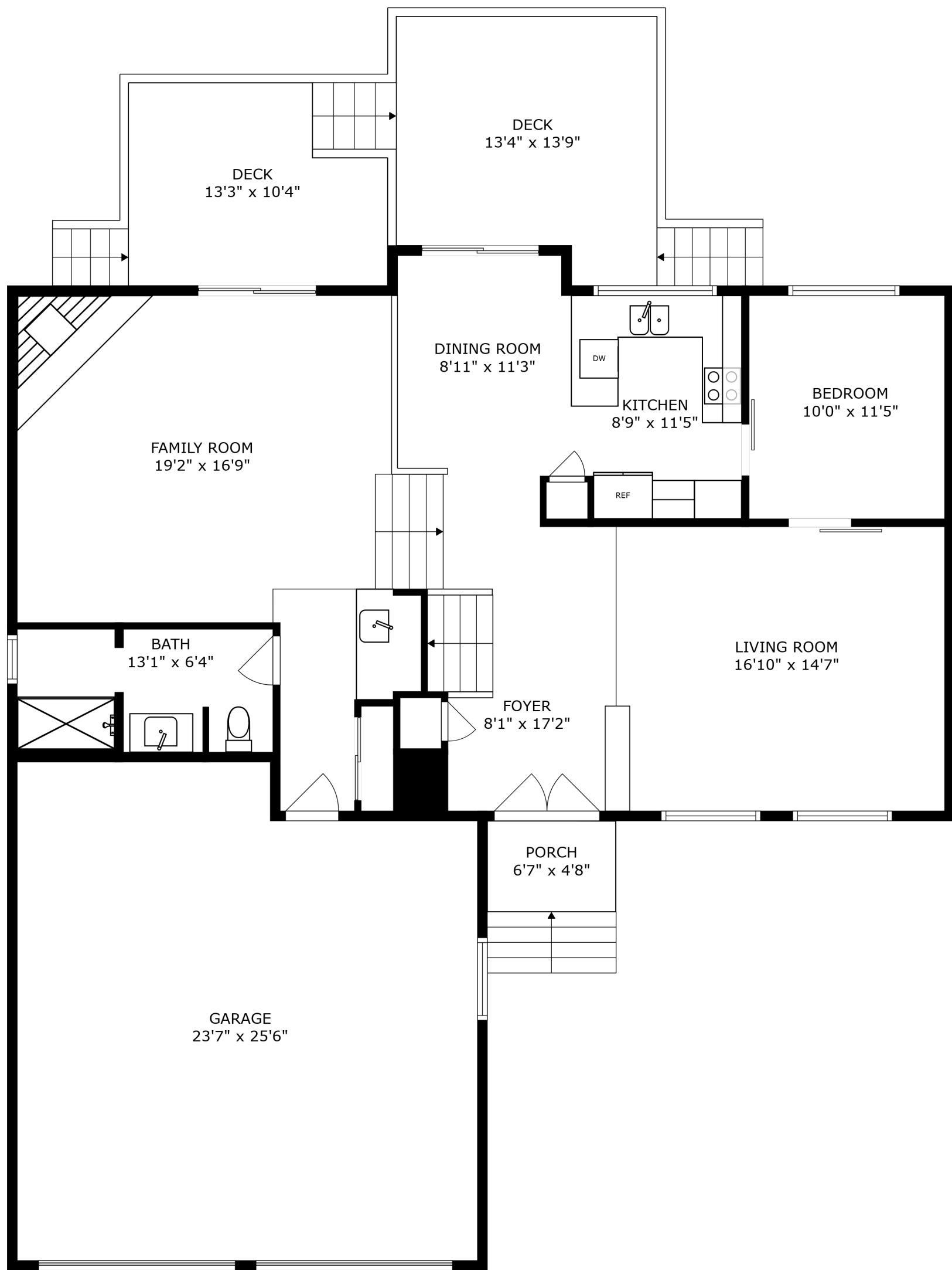
FLOOR 1
