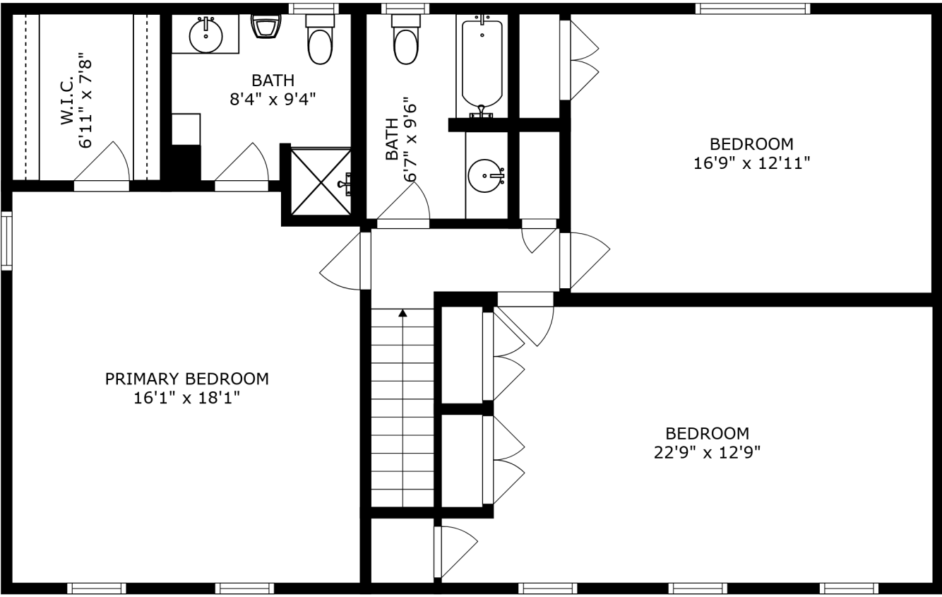
FLOOR 3
