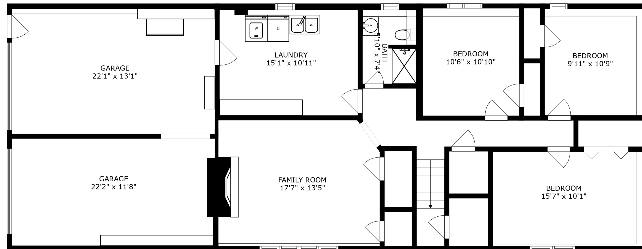
FLOOR 1
