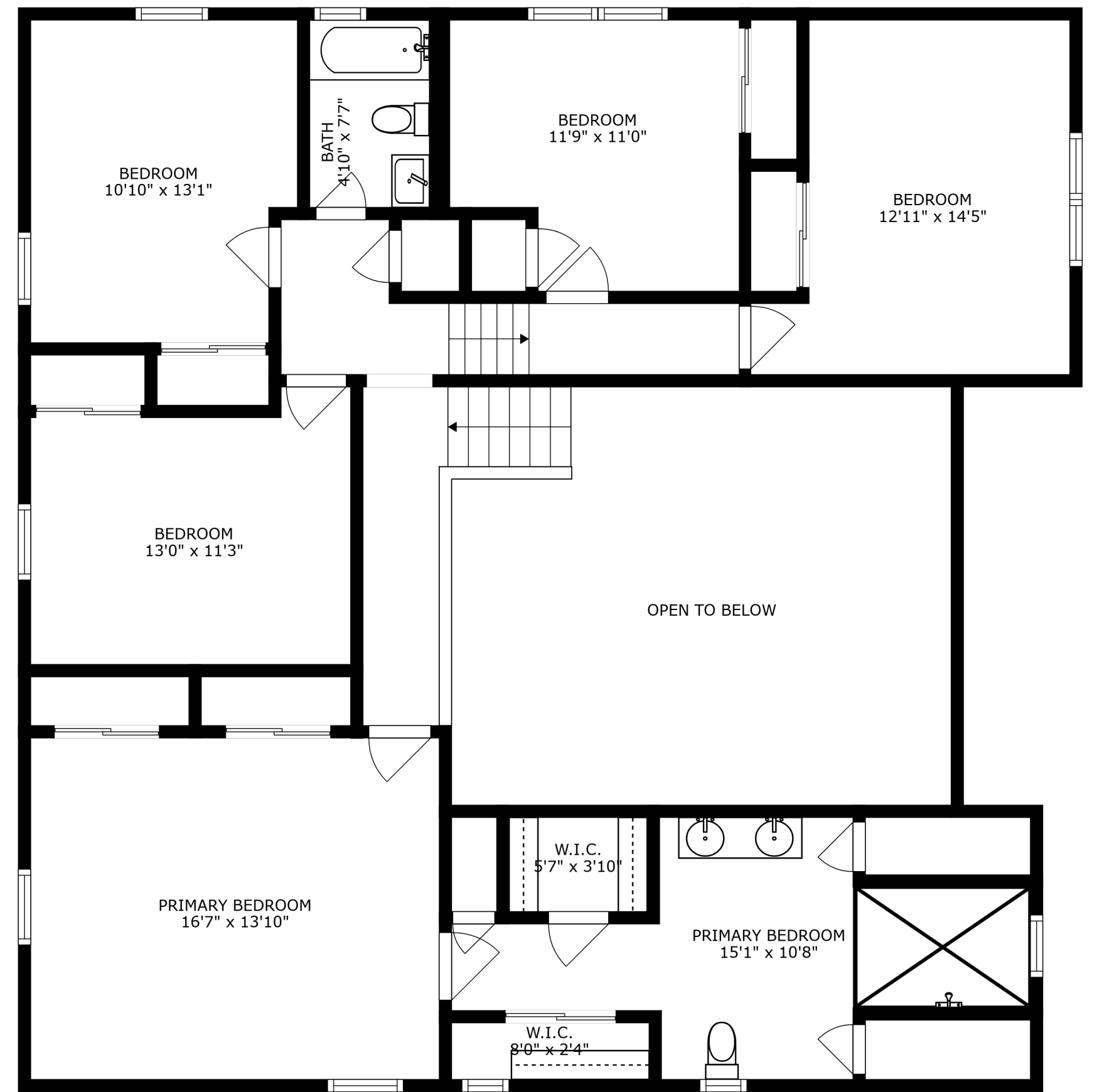
FLOOR 2
