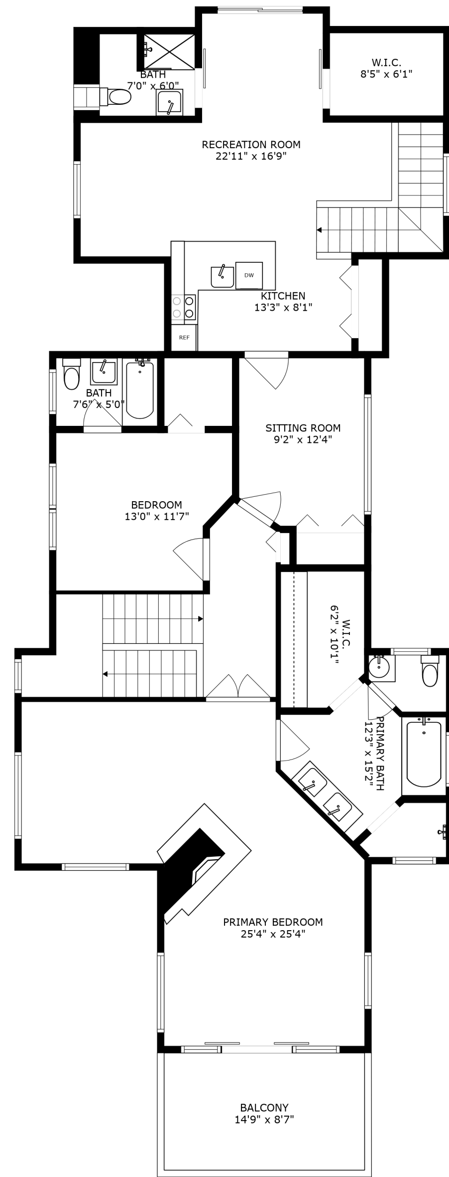
FLOOR 3
