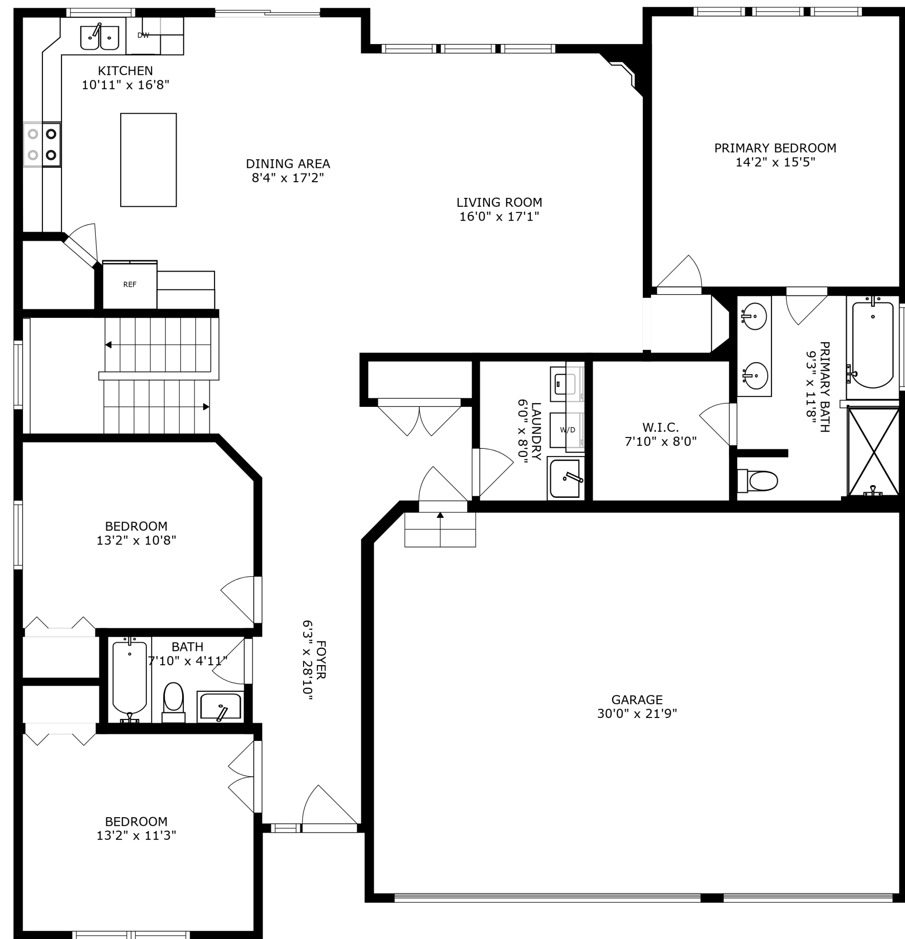
FLOOR 2
