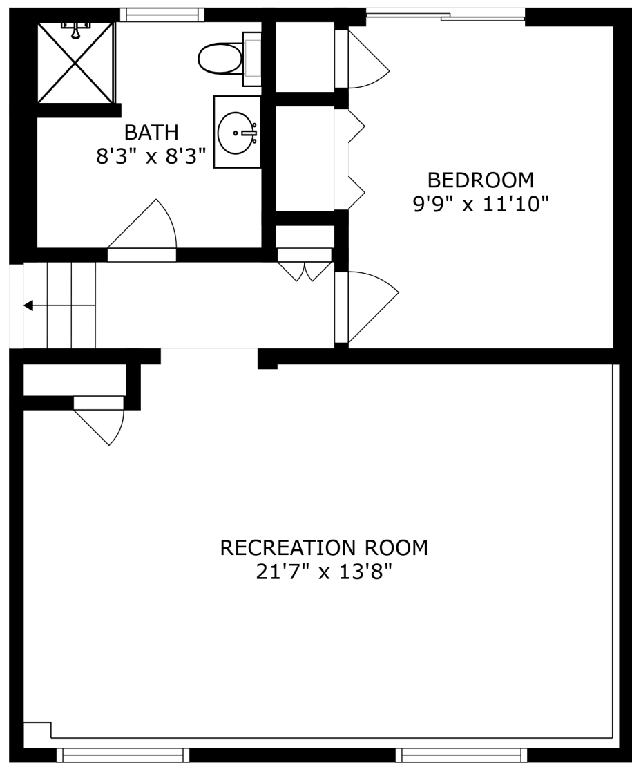
FLOOR 1
