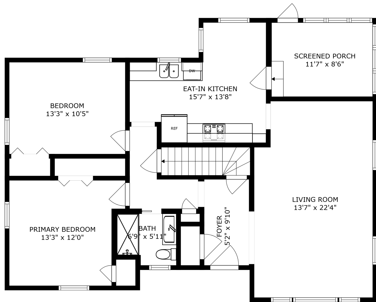
FLOOR 2
