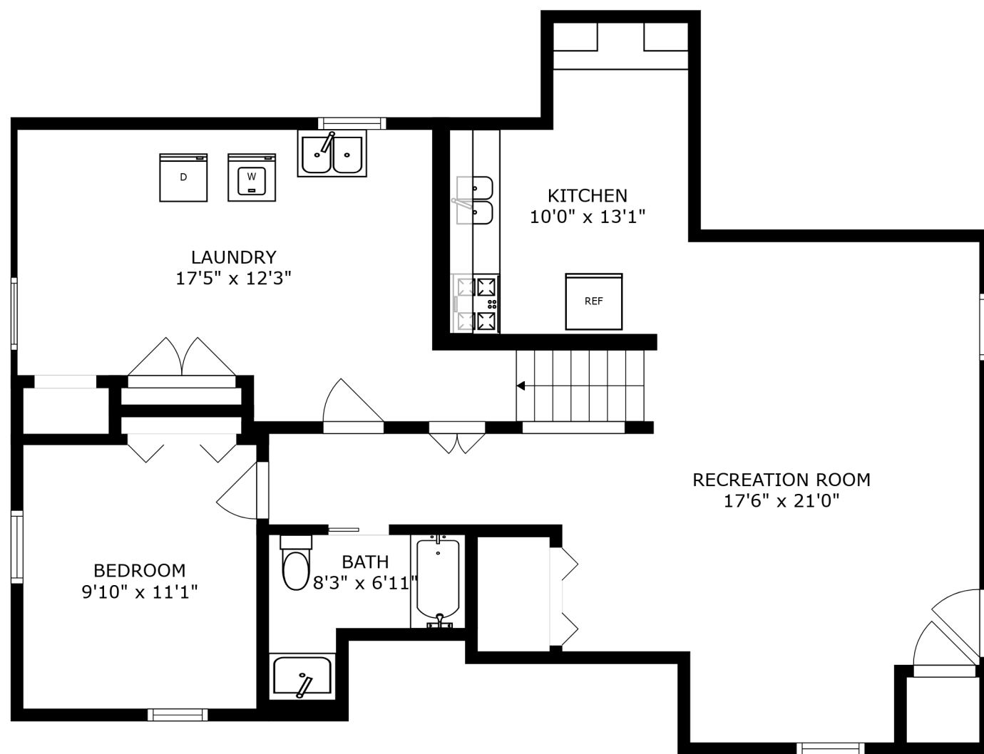
FLOOR 1
