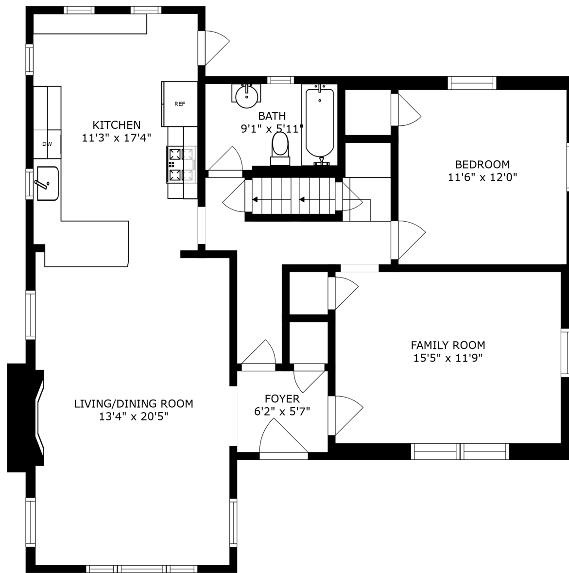
FLOOR 2
