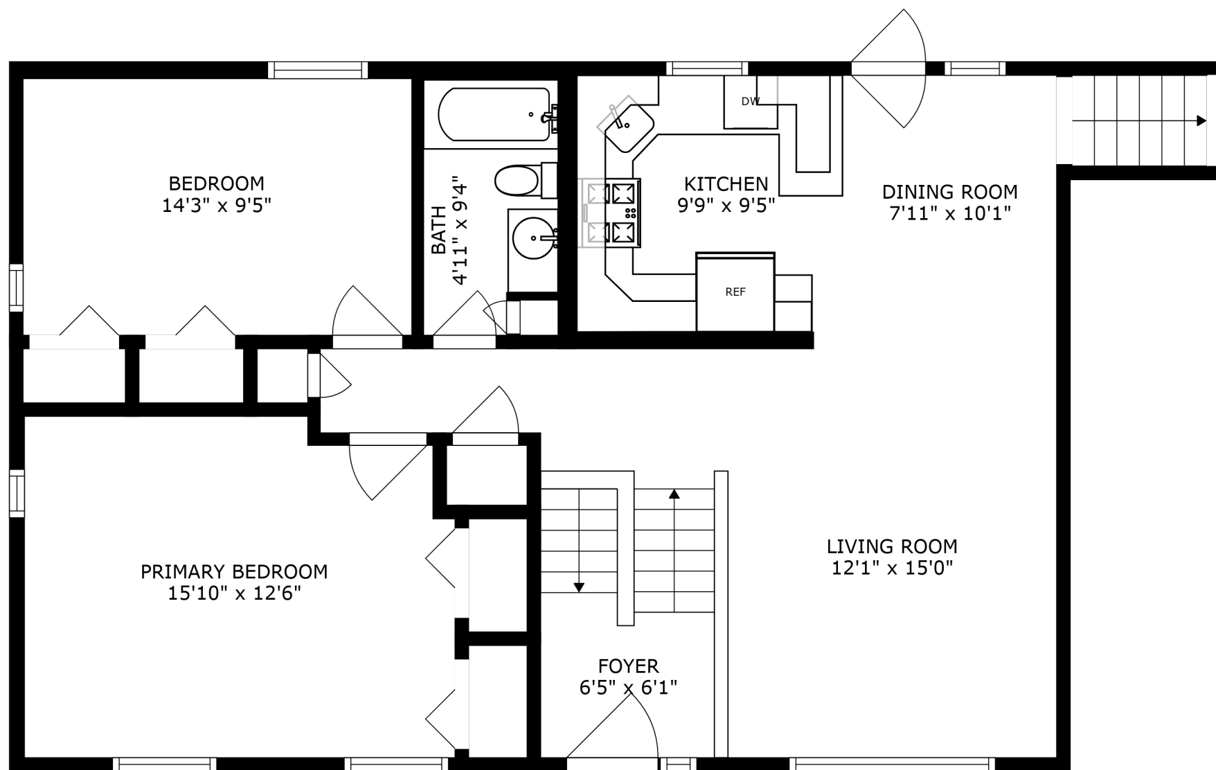
FLOOR 2
