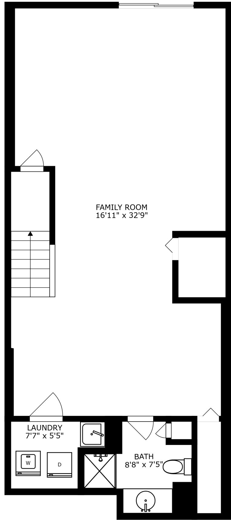
FLOOR 1
