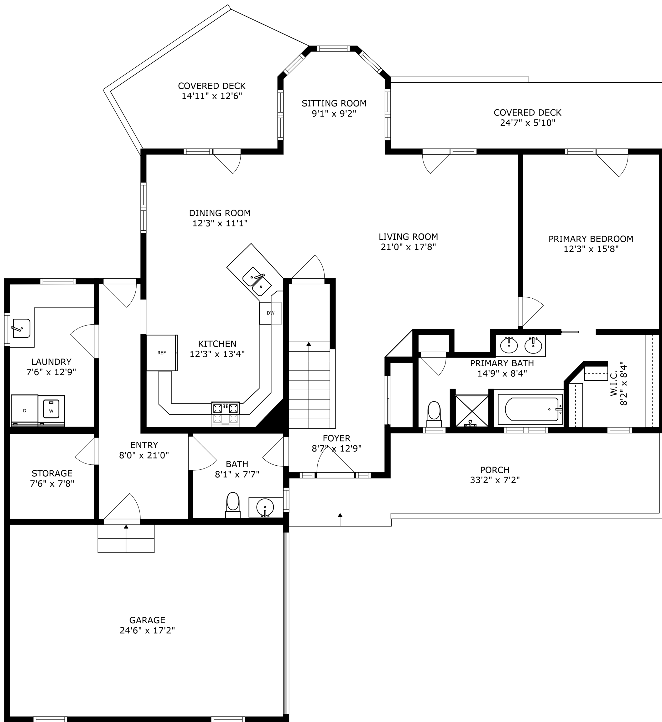
FLOOR 1
