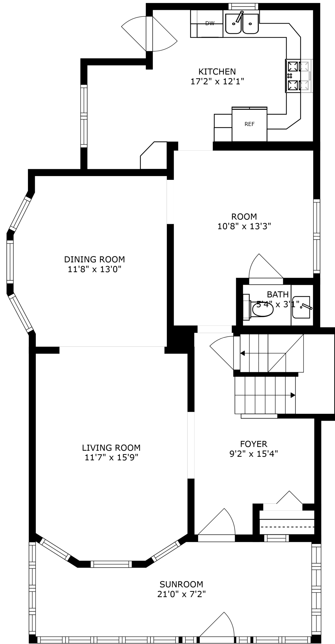
FLOOR 2
