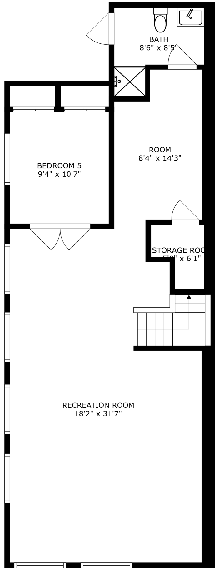
FLOOR 1
