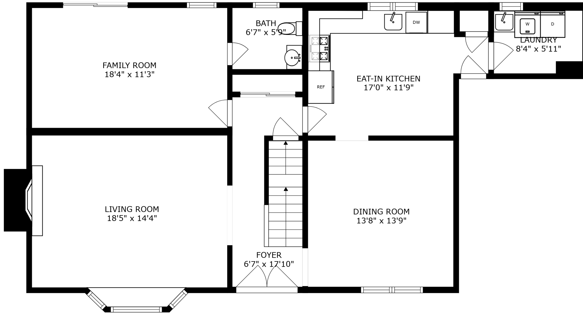
FLOOR 2
