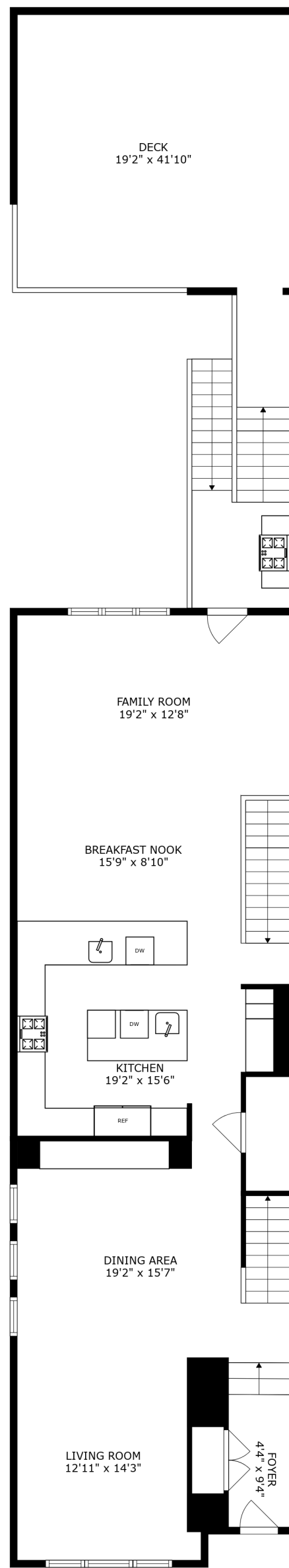
FLOOR 2
