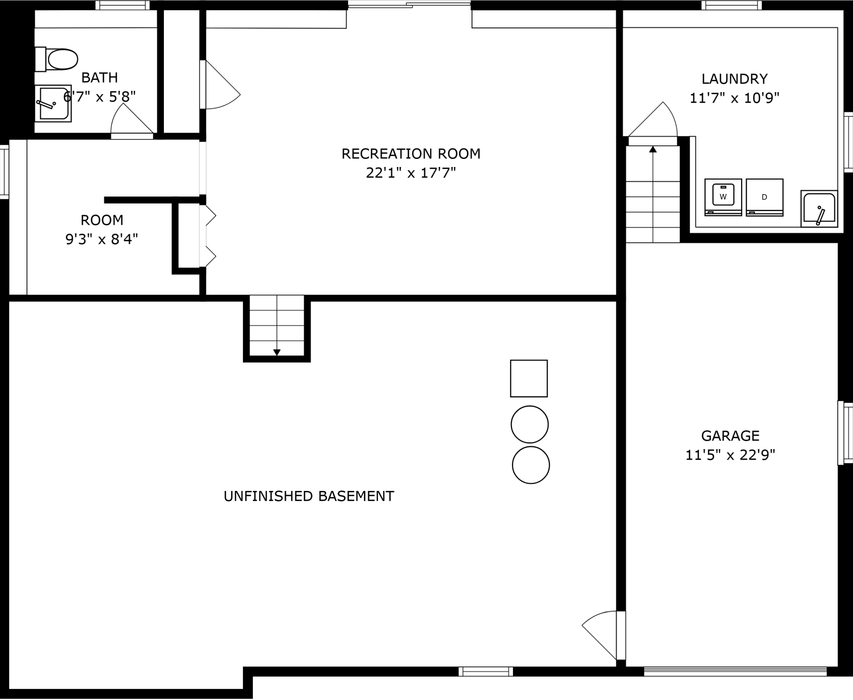
FLOOR 1
