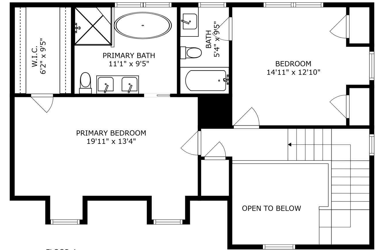
FLOOR 4
