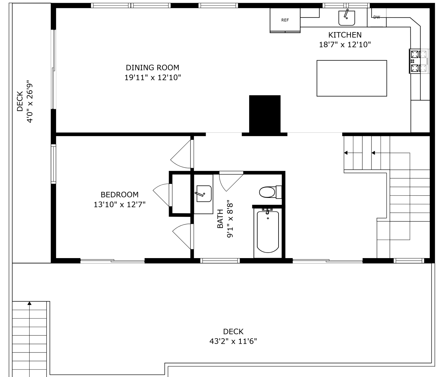
FLOOR 3
