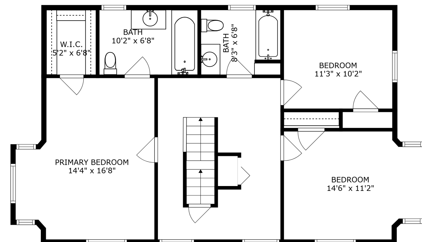
FLOOR 3
