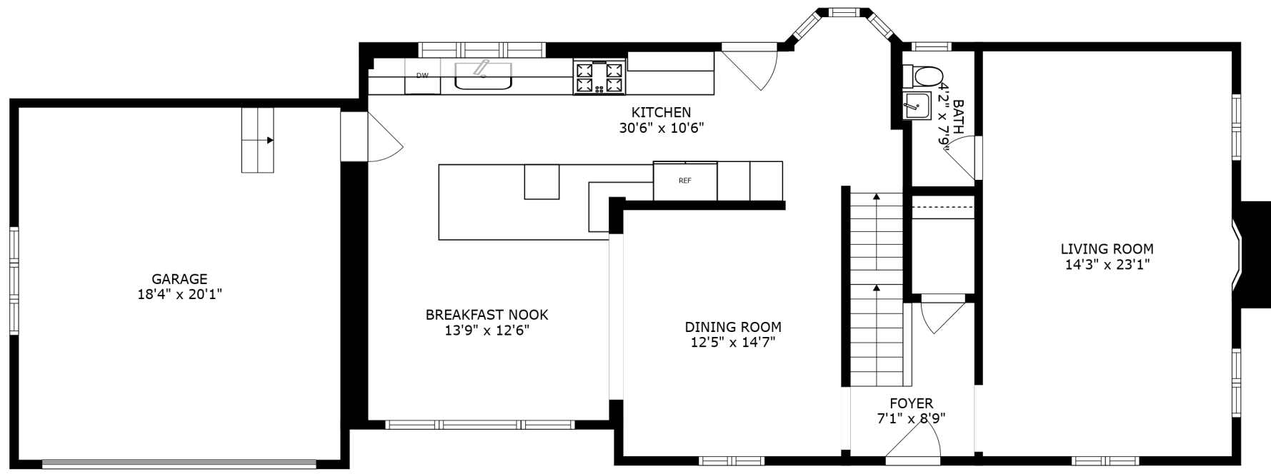
FLOOR 2
