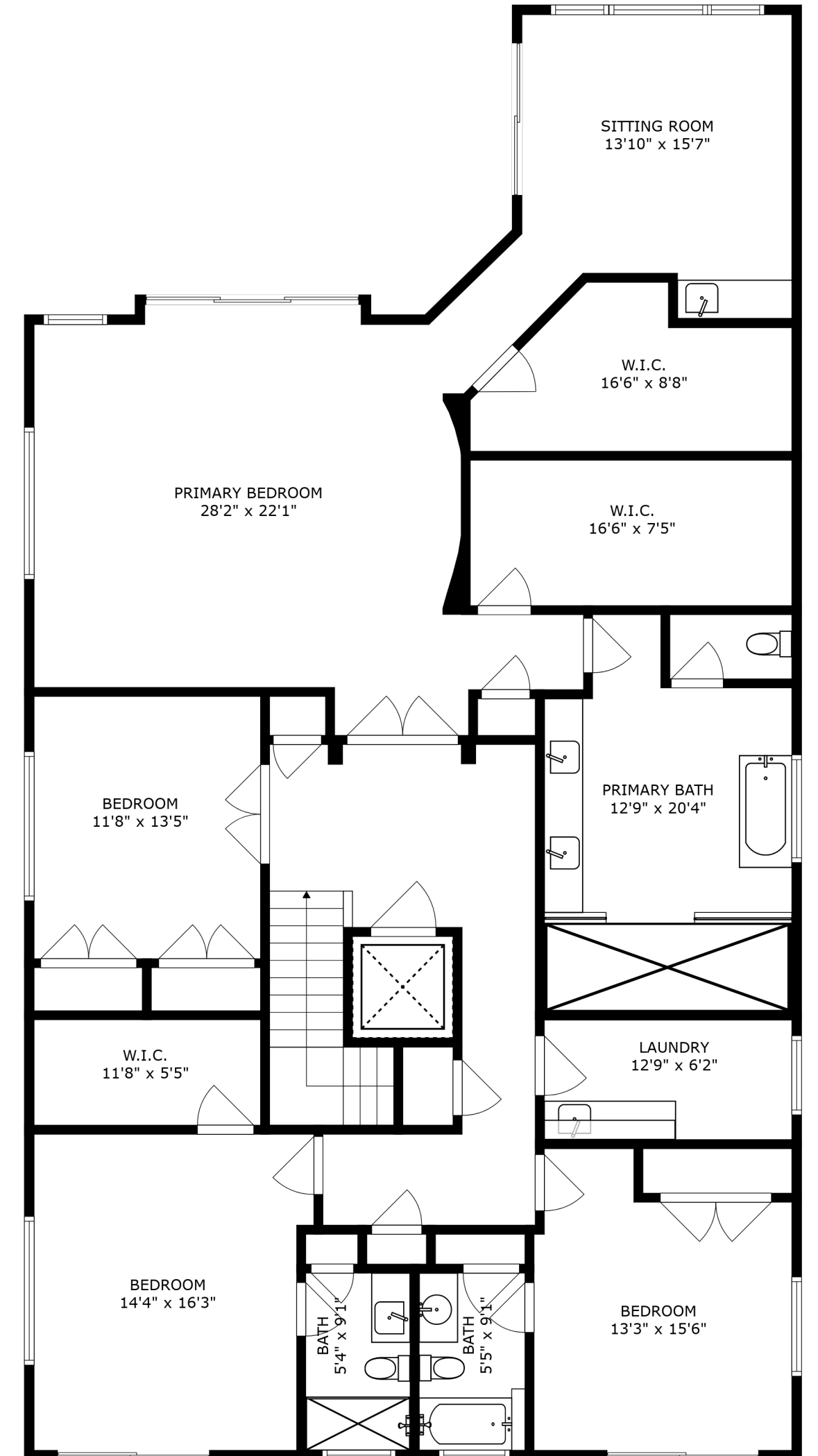
FLOOR 3
