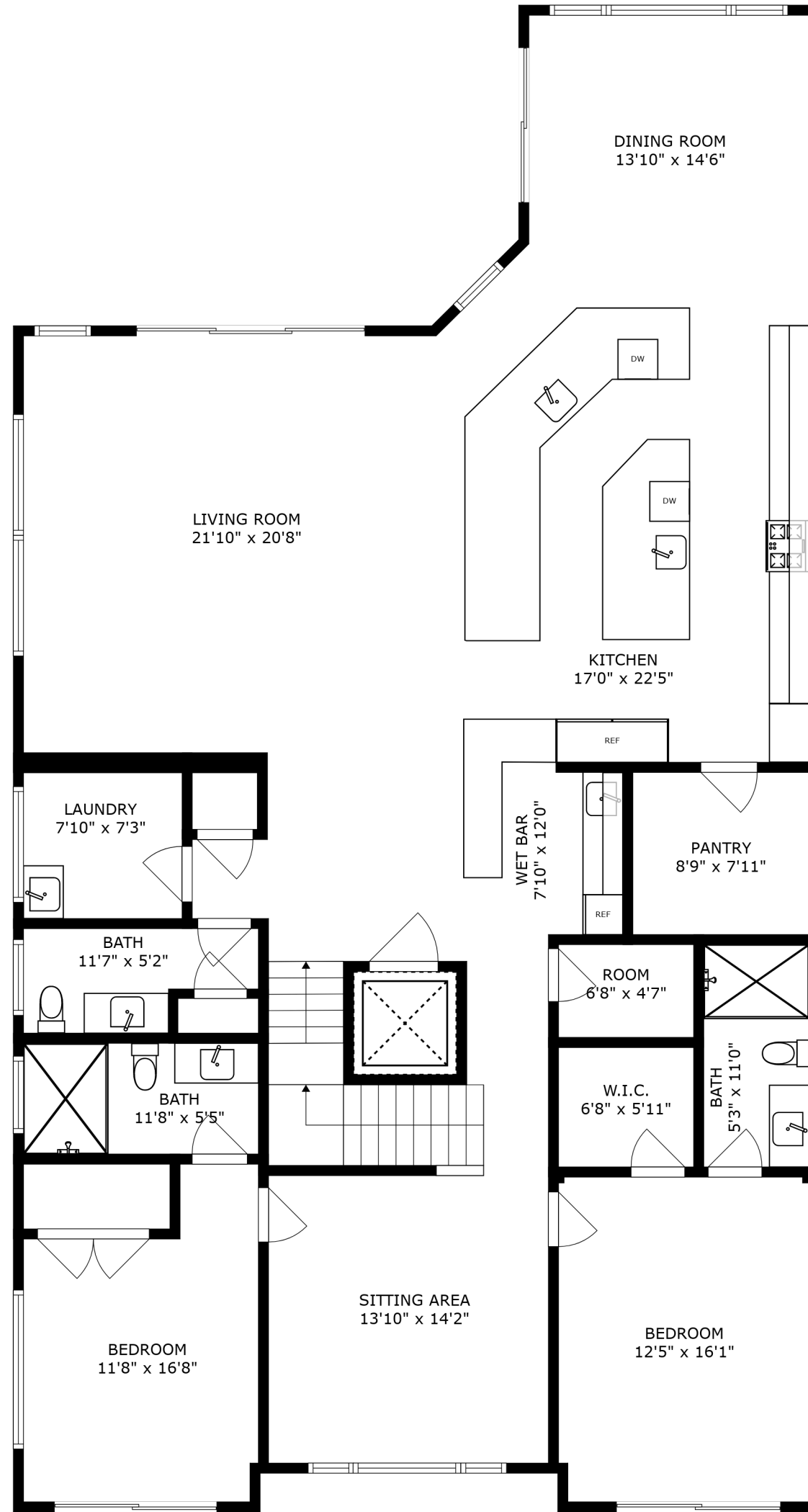
FLOOR 2
