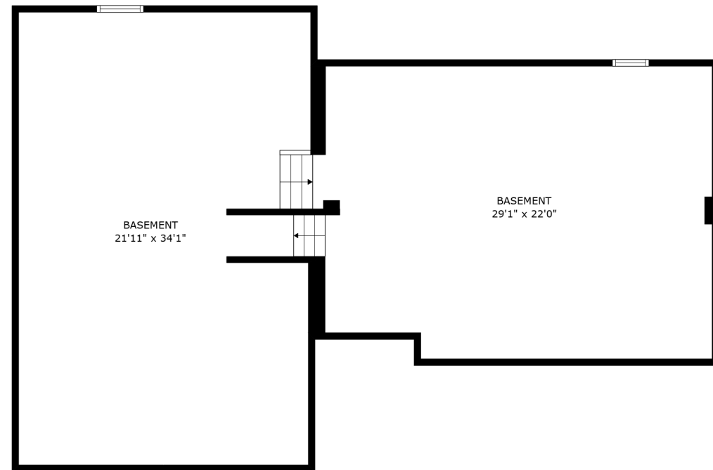
FLOOR 1
