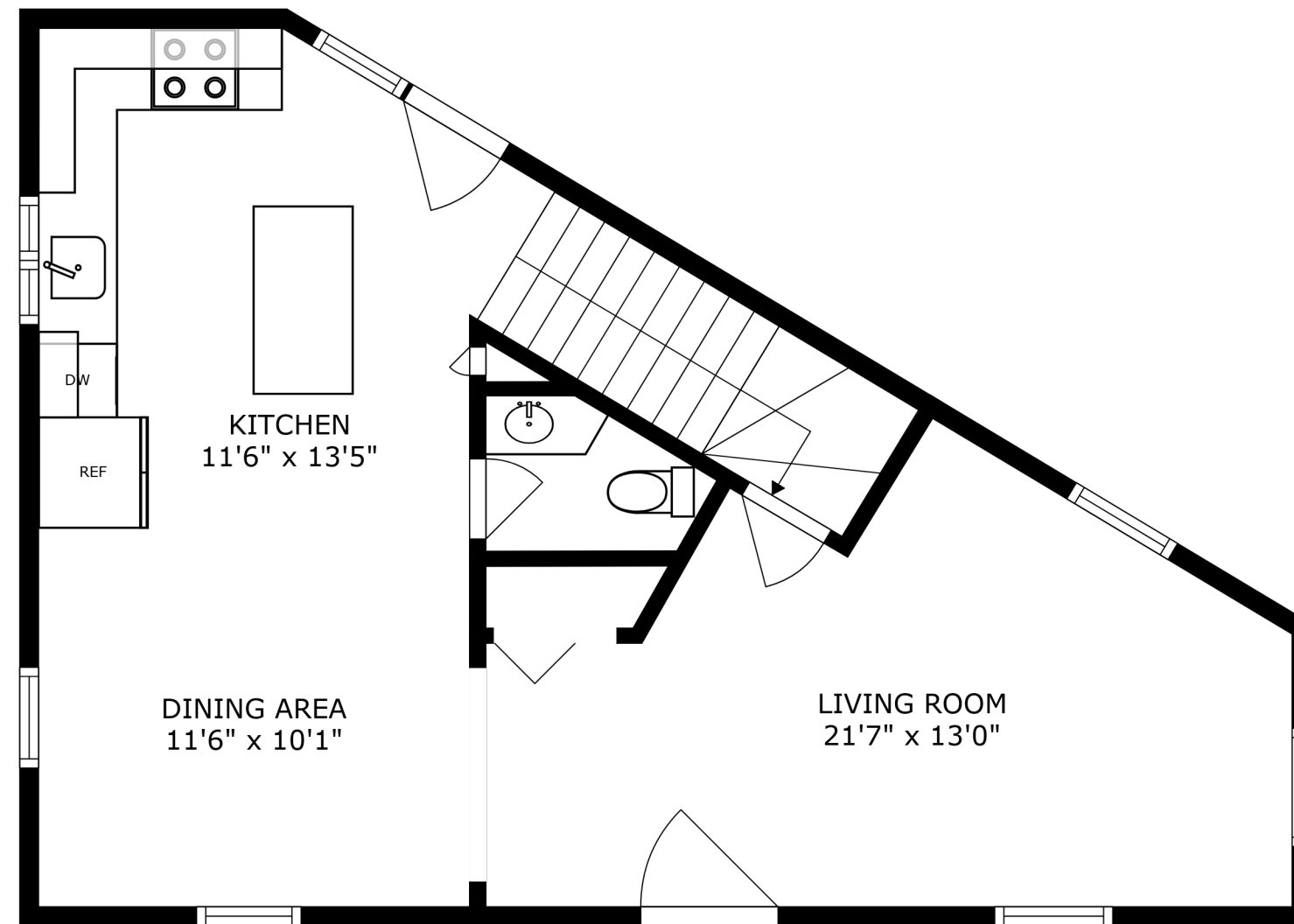
FLOOR 3
