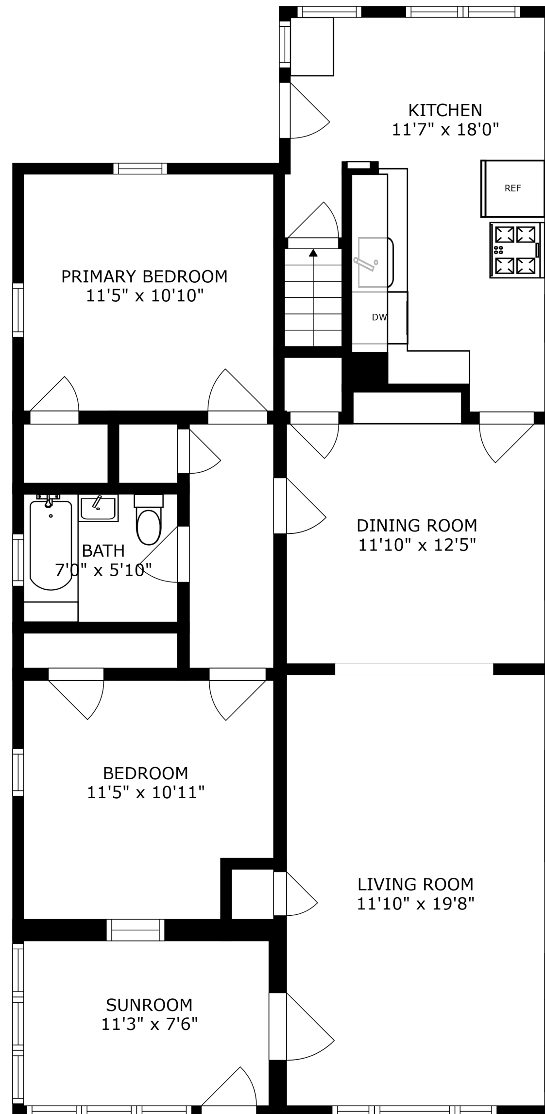
FLOOR 2
