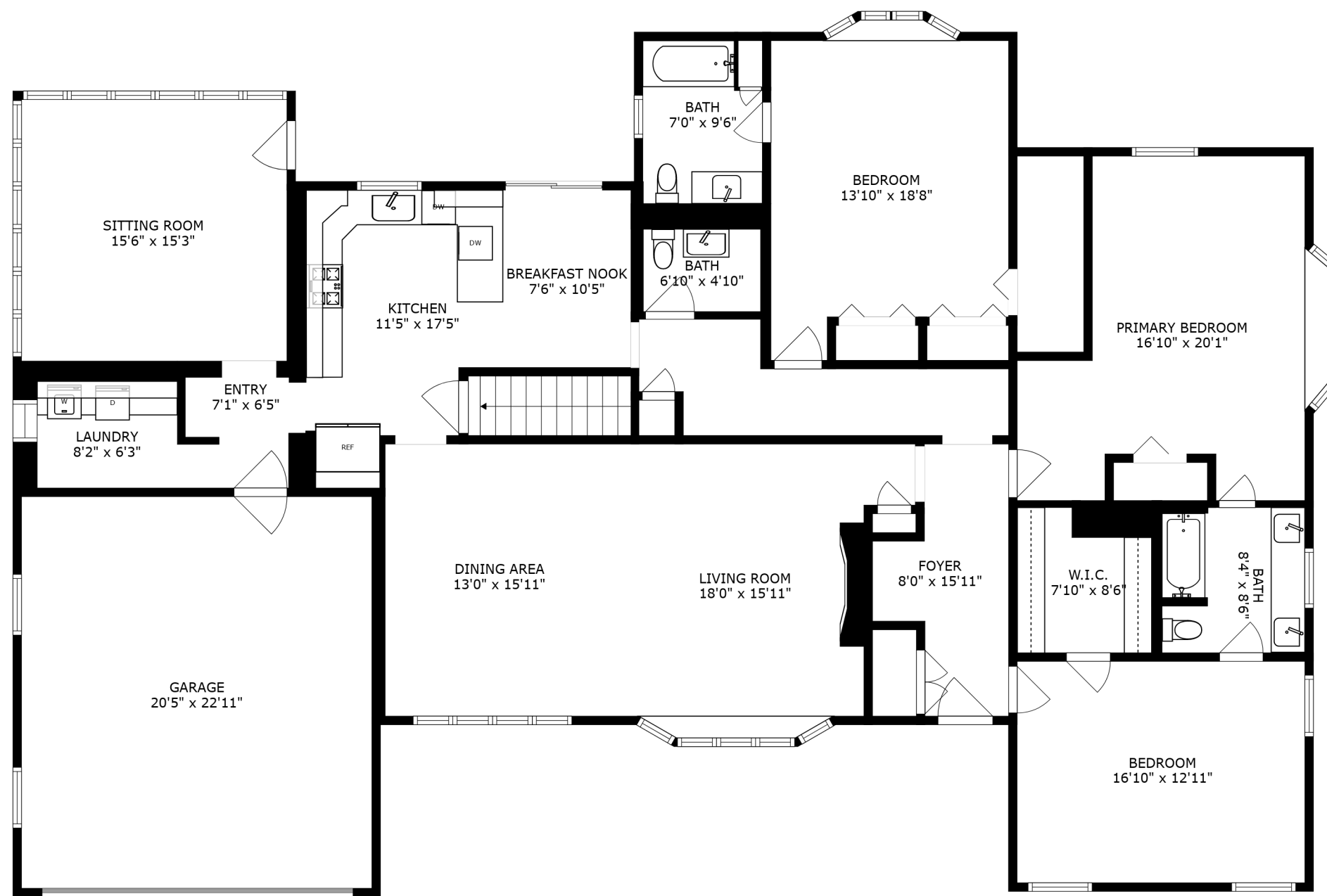
FLOOR 2
