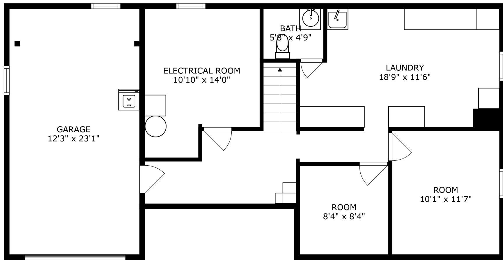
FLOOR 1
