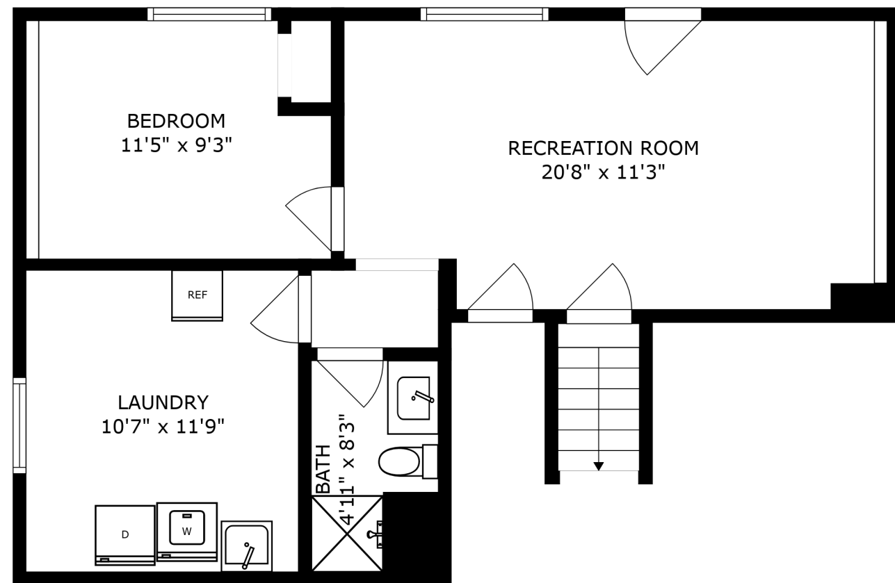
FLOOR 1
