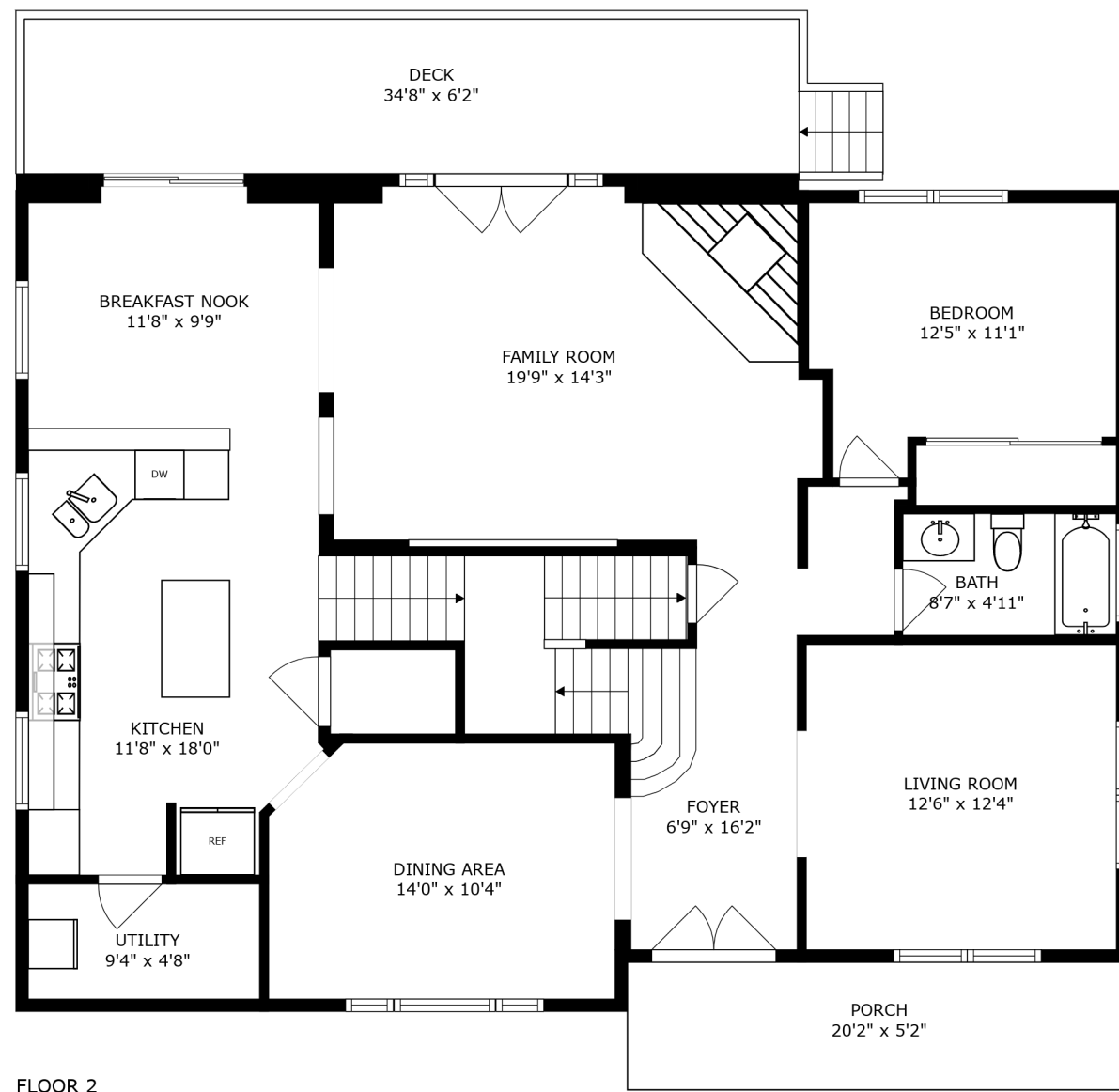
FLOOR 2
