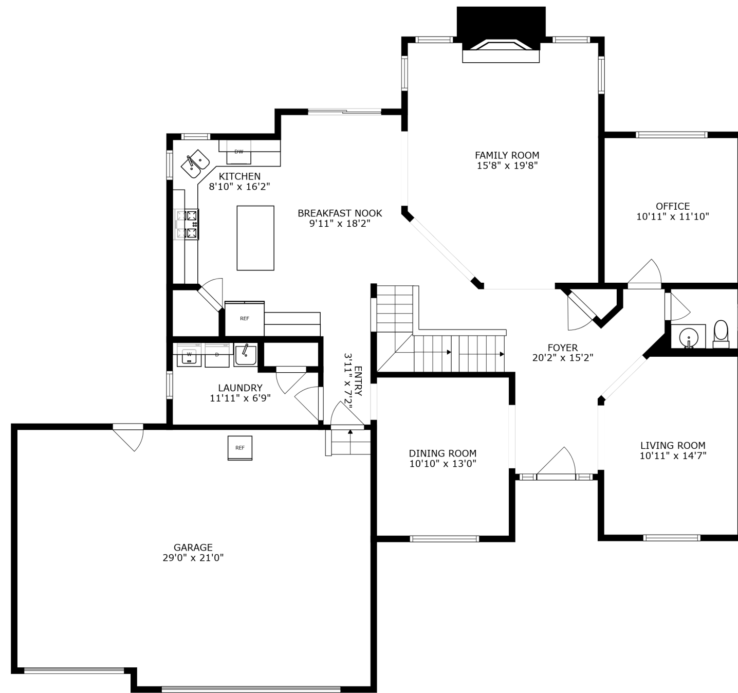
FLOOR 2
