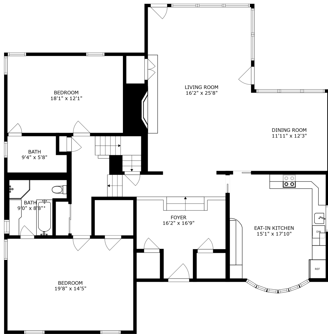
FLOOR 2
