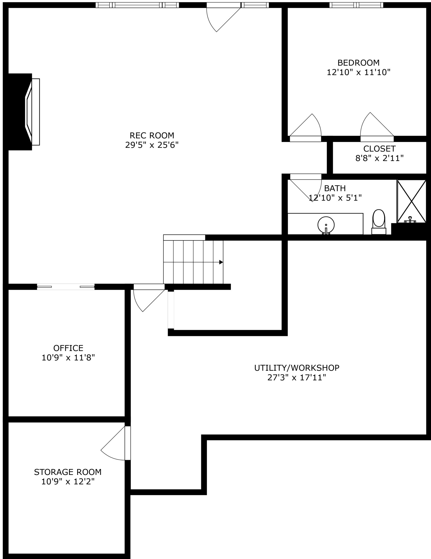
FLOOR 1
