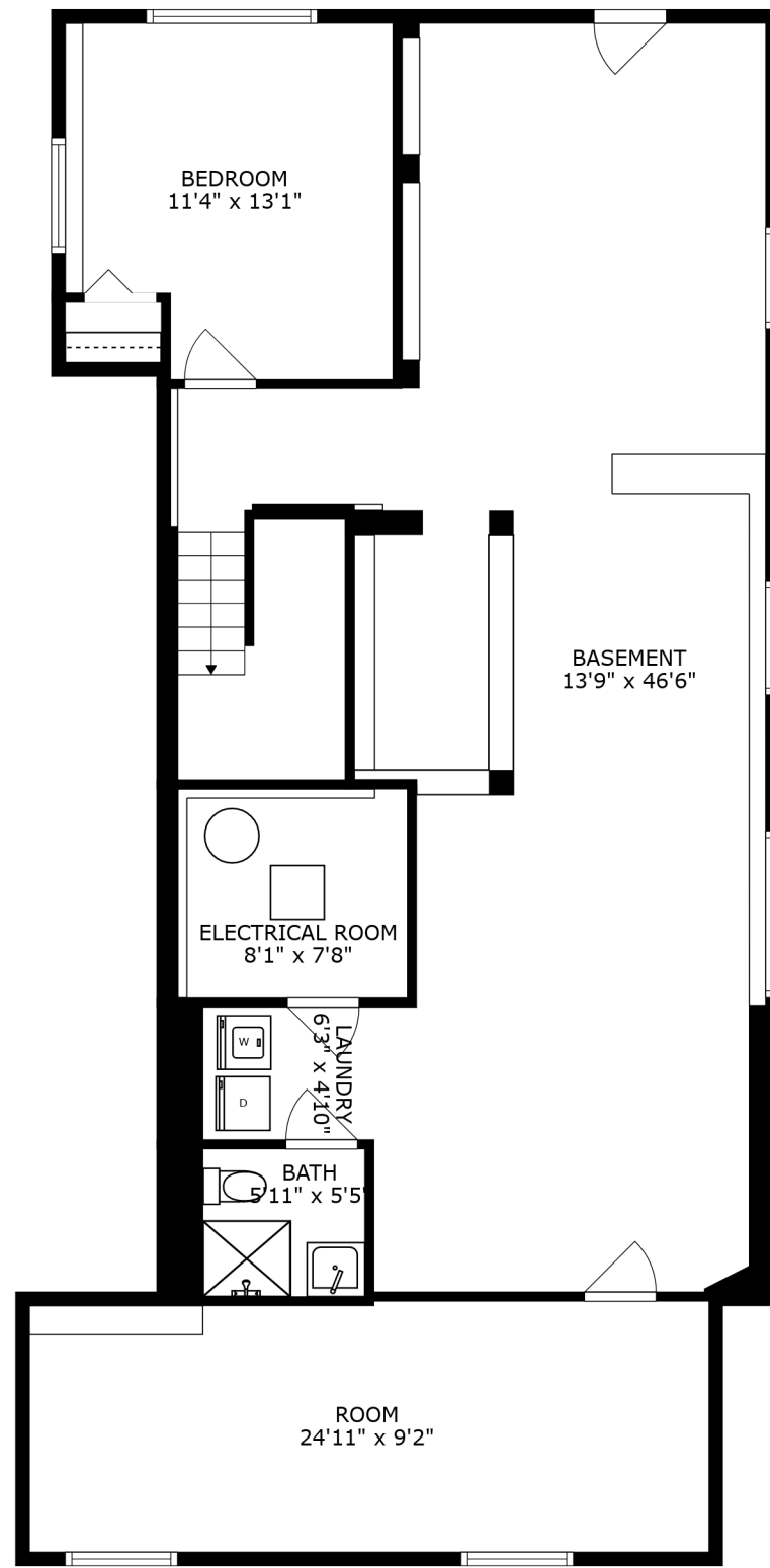
FLOOR 1
