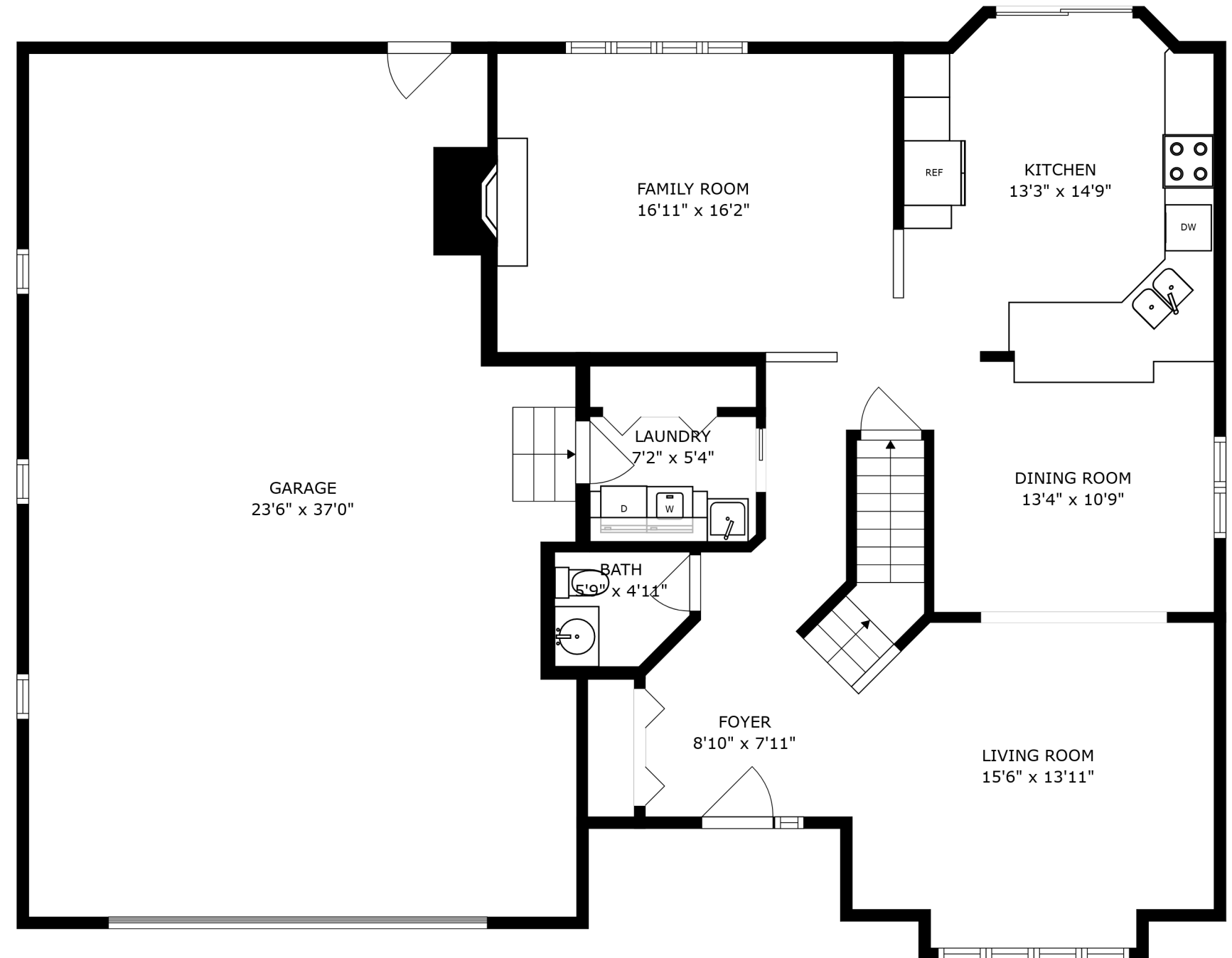
FLOOR 2
