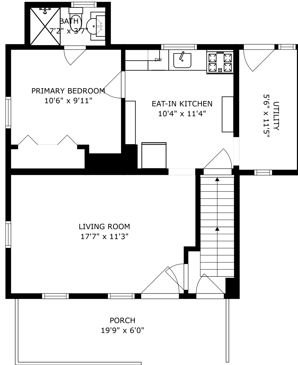
FLOOR 2
