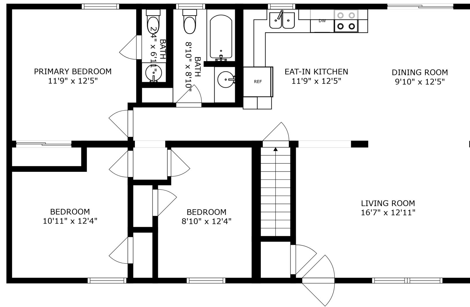
FLOOR 2
