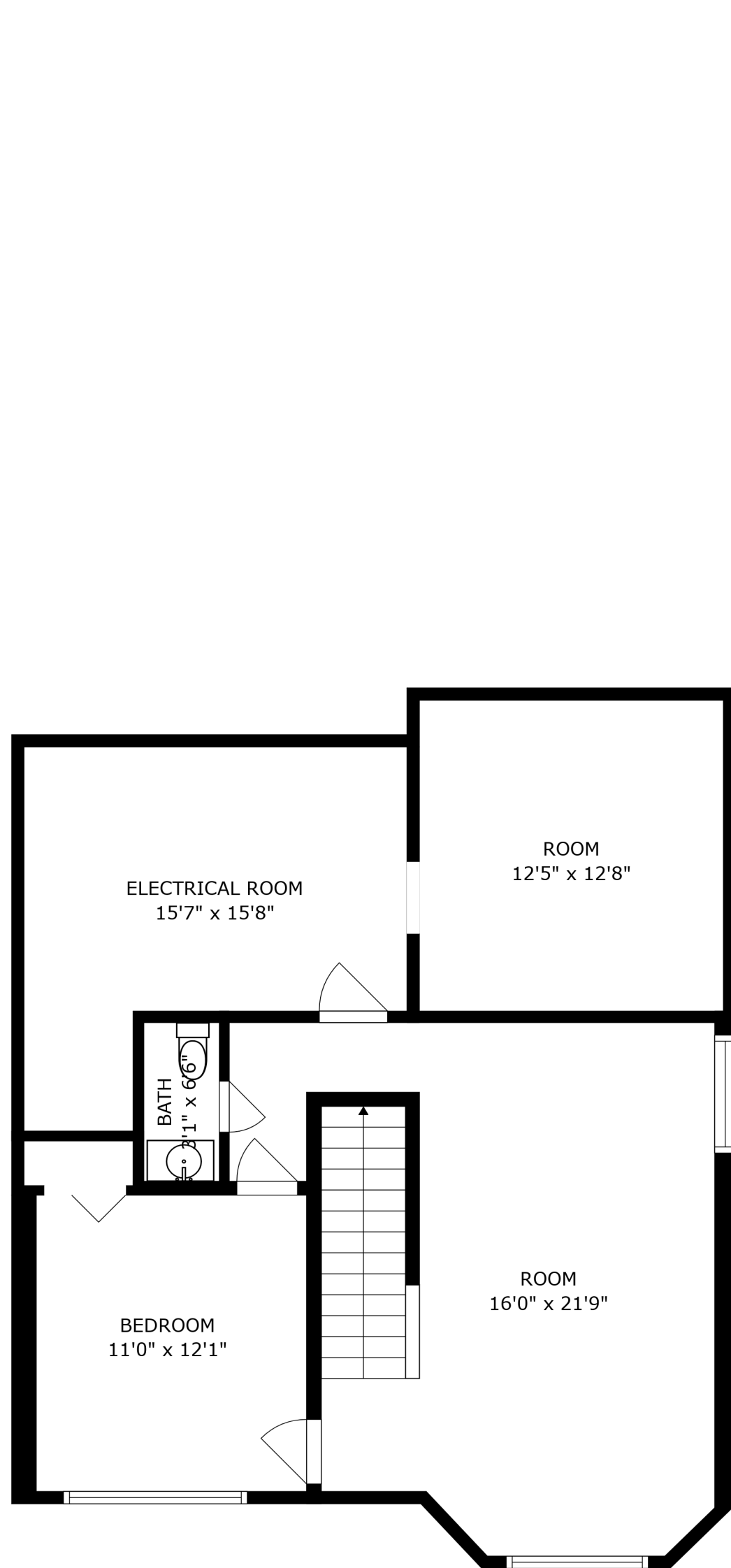
FLOOR 1
