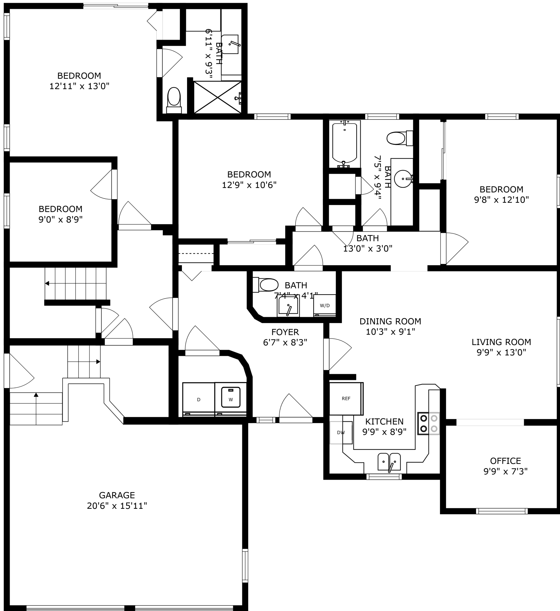
FLOOR 1
