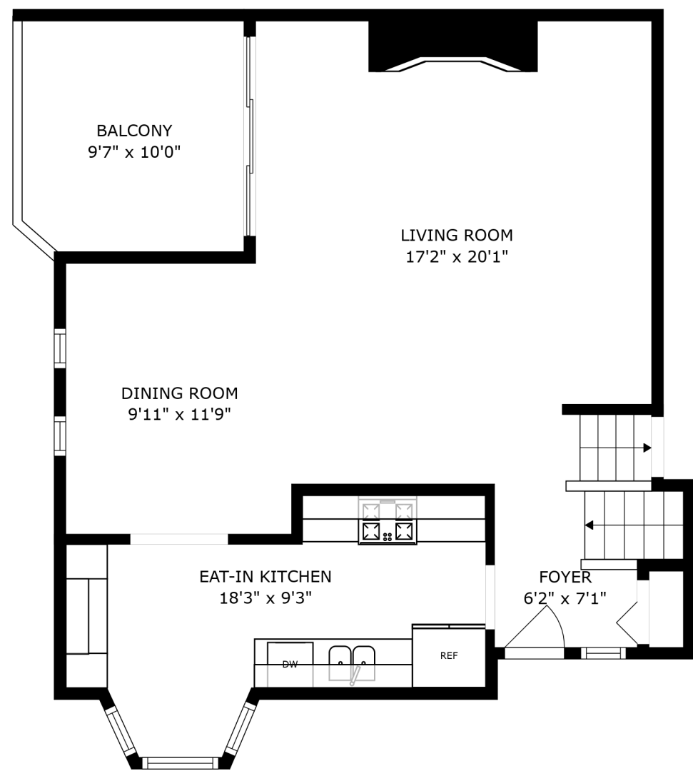
FLOOR 3
