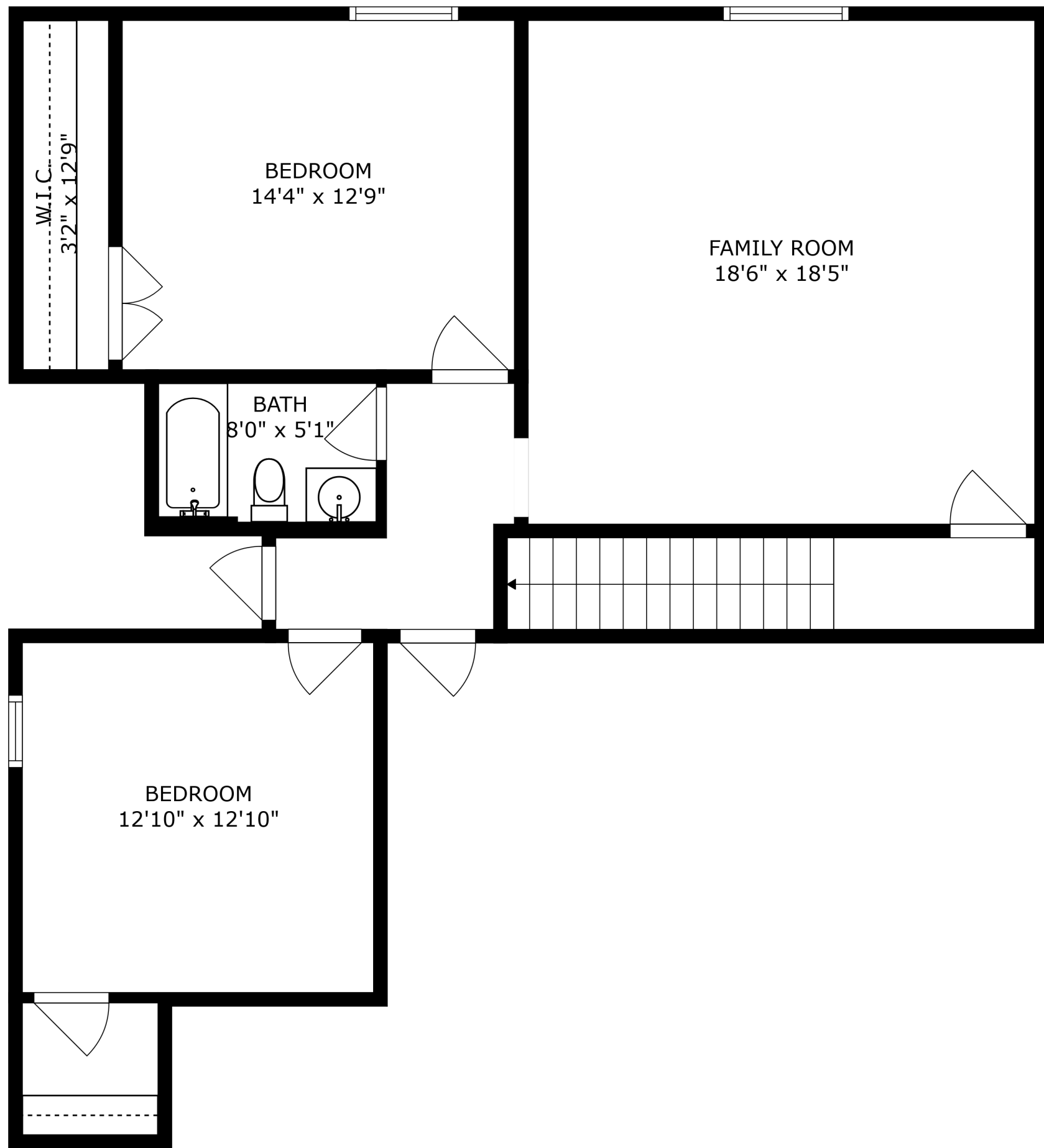
FLOOR 1
