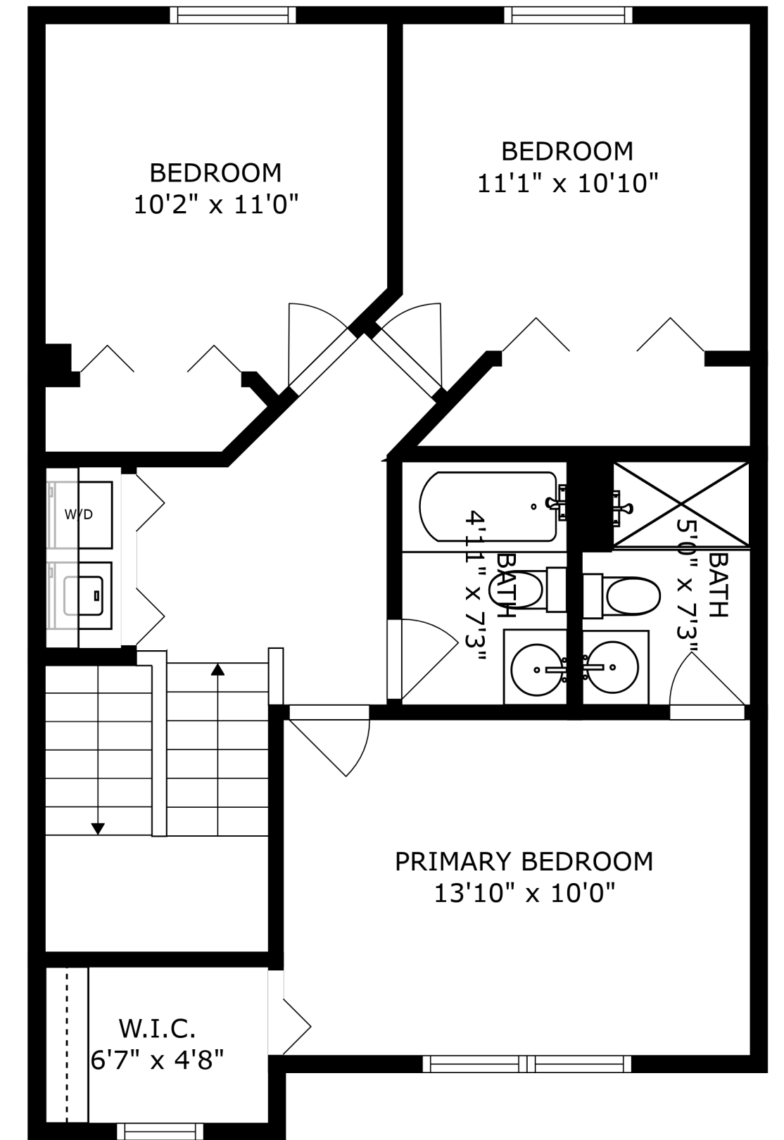
FLOOR 3
