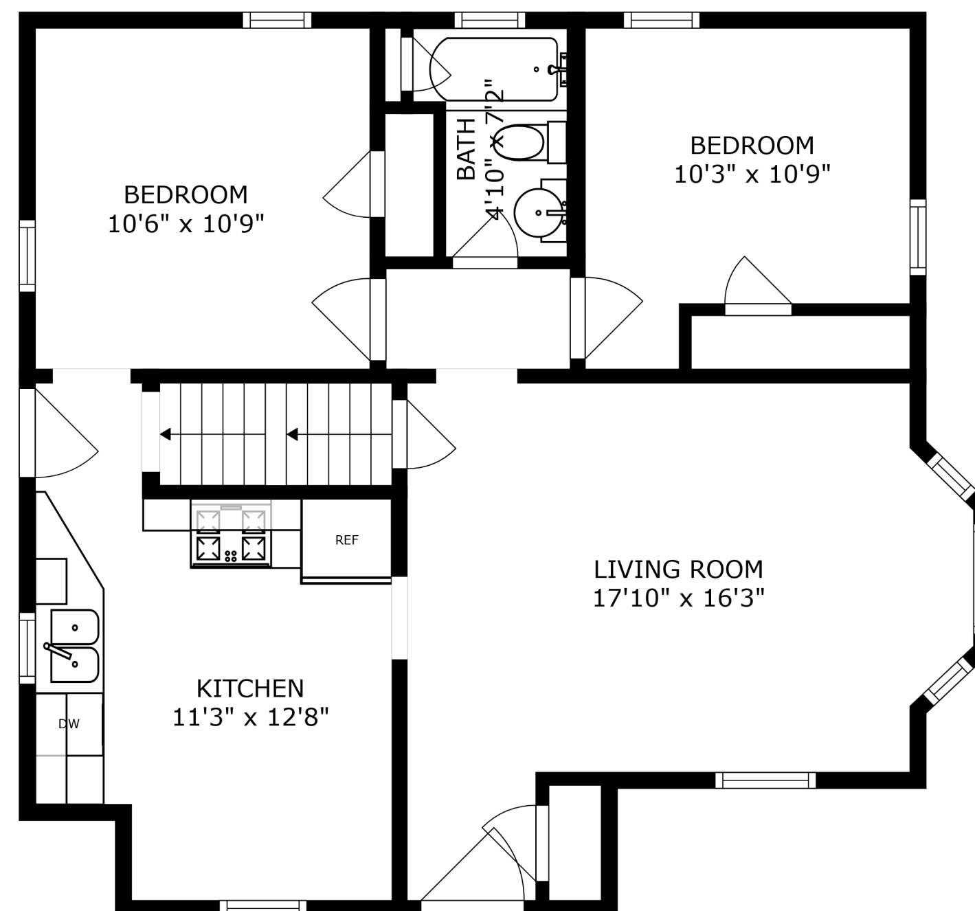
FLOOR 2
