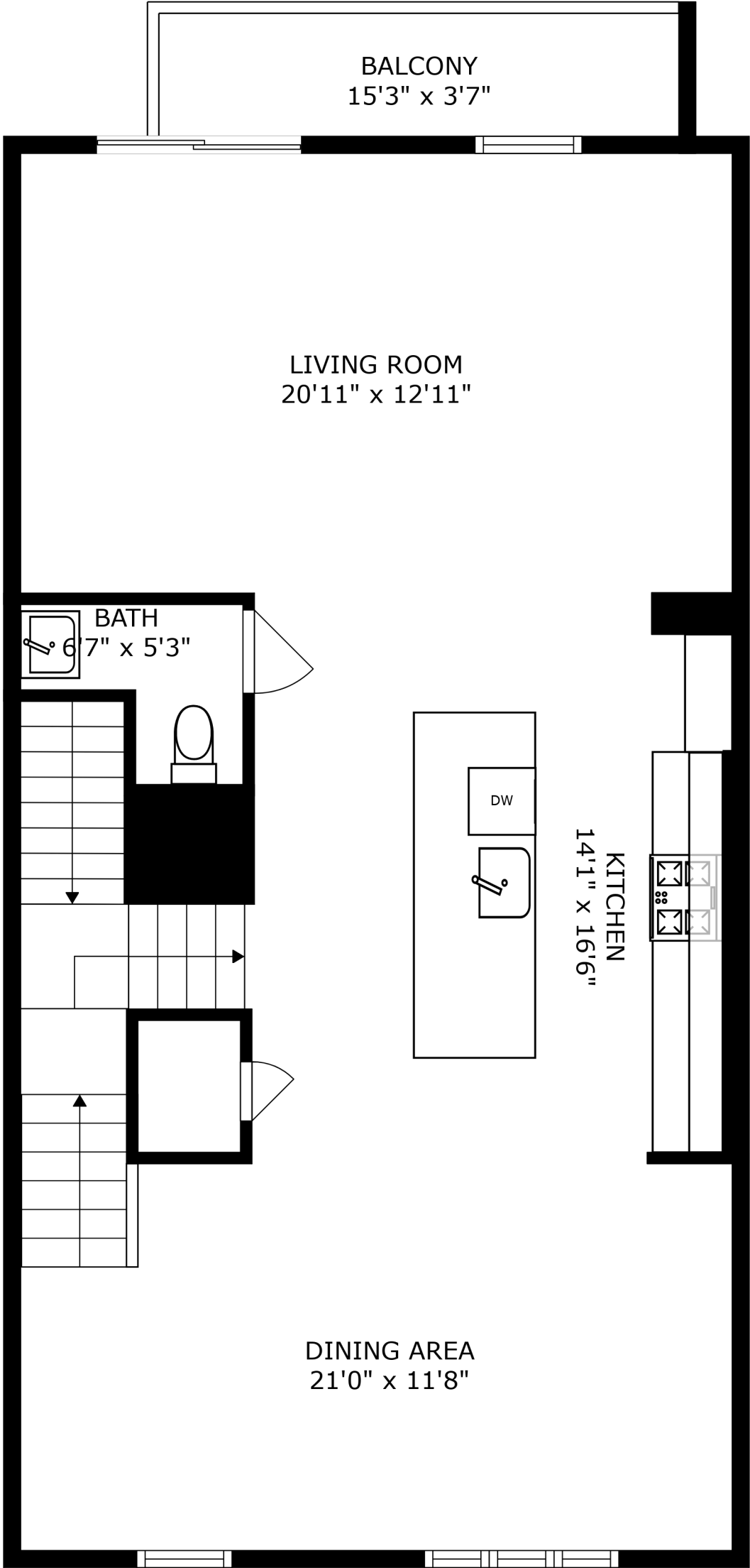
FLOOR 2
