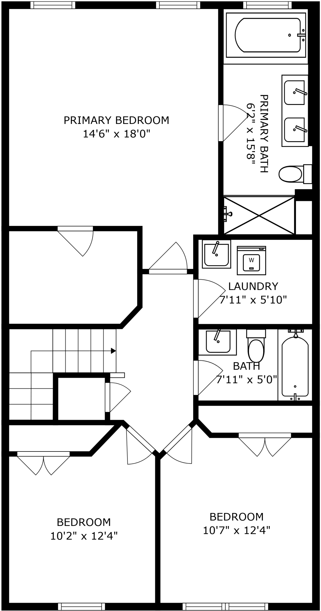
FLOOR 3
