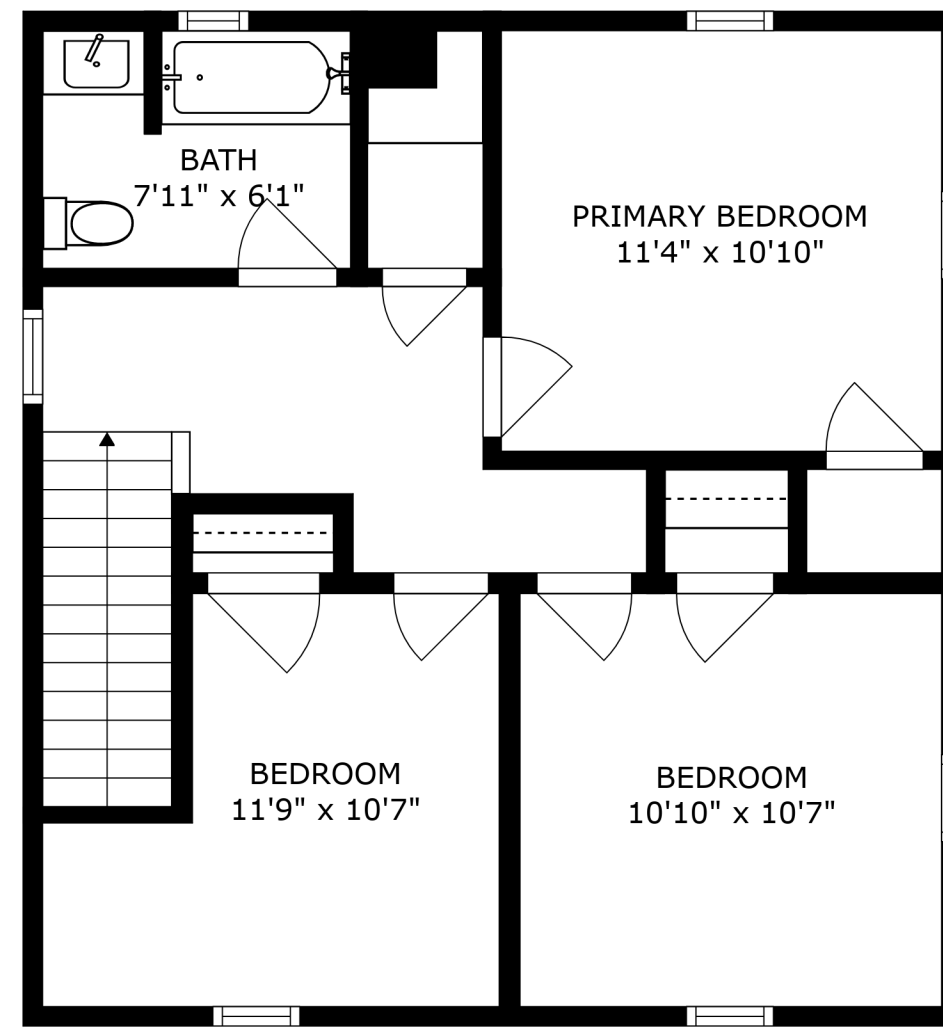
FLOOR 3
